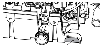
Thinned bottom cable entry section on the Backplate .
